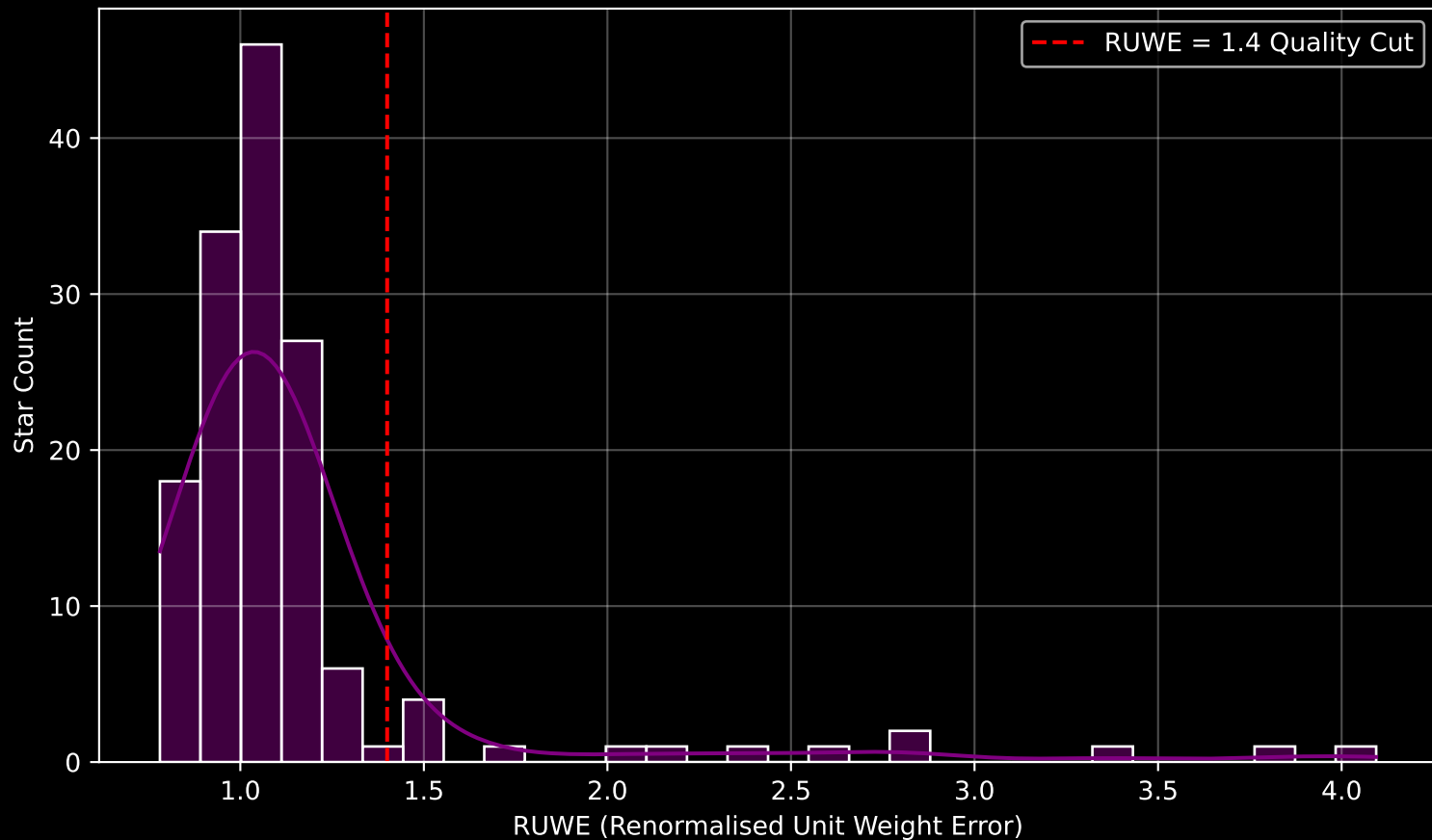
GALAH DR4 Field [7211] RUWE Distribution (n= 146)
