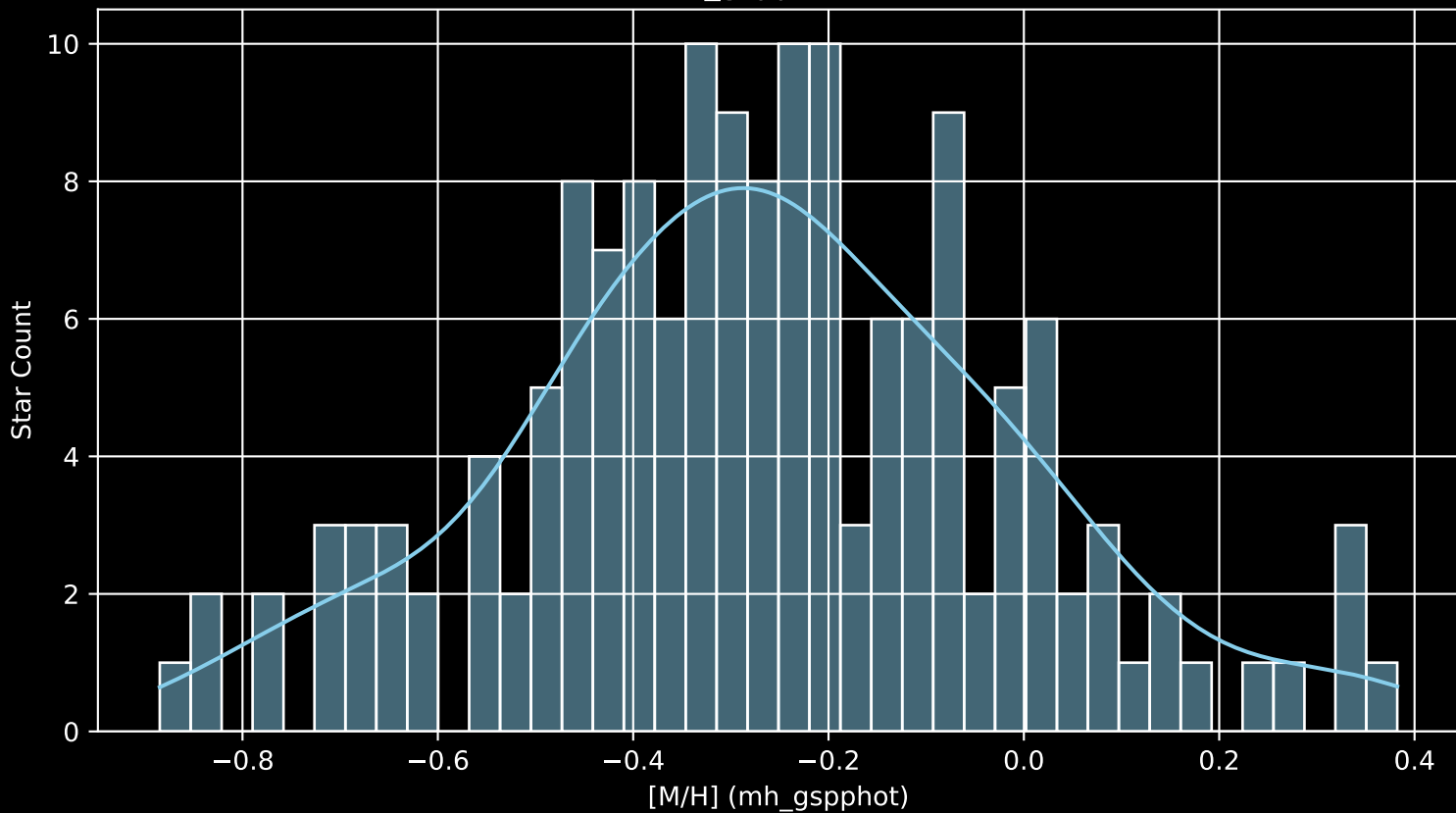
GALAH DR4 Field: [7211] [M/H] (mh_gspphot) (n= 155)
