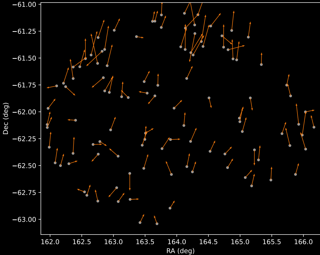
GALAH DR4 Cluster 2 Proper Motion Vectors (n=108)
