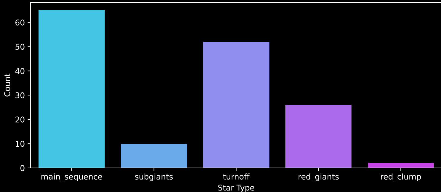
GALAH DR4 Field: [7211] Count plot of Star Type
