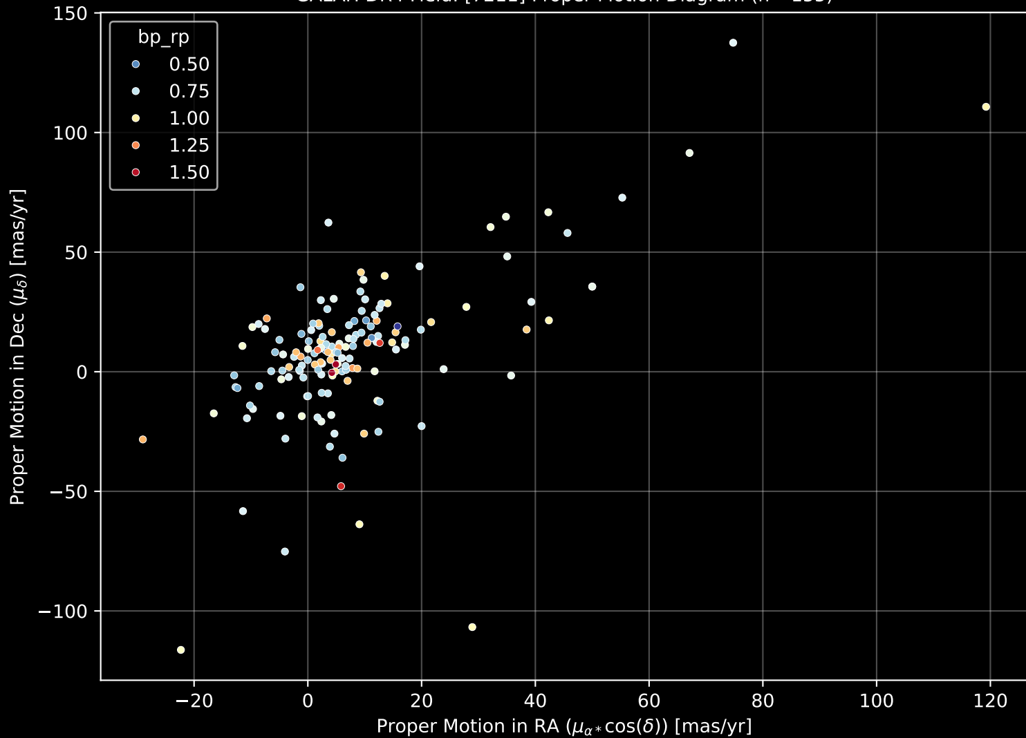
GALAH DR4 Field: [7211] Proper Motion Diagram (n= 155)
