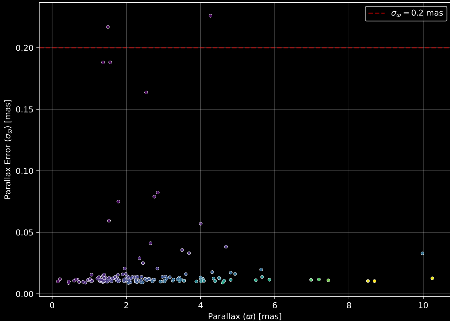
GALAH DR4 Field: [7211] Parallax Quality (n= 155)
