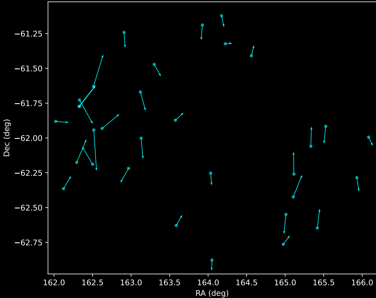
GALAH DR4 Noise Stream Proper Motion Vectors (n=32)
